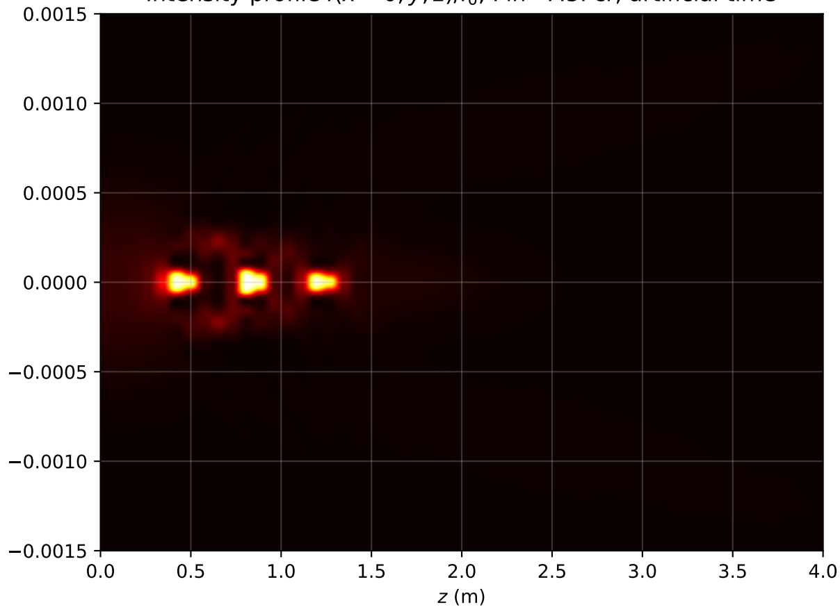
Intensity profile I(x=0, y, z)/I_0 , P_{in}=7.5P_{cr} , artificial time
